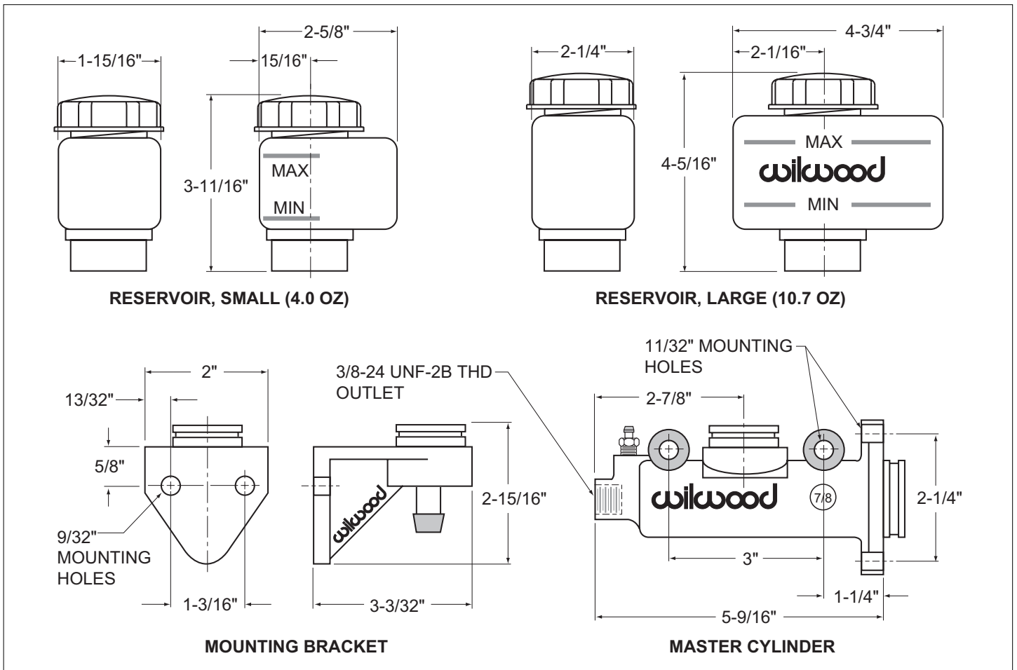
Figure 3. Minimum Mounting Requirements for Mounting Bracket, Master Cylinder and Reservoirs
