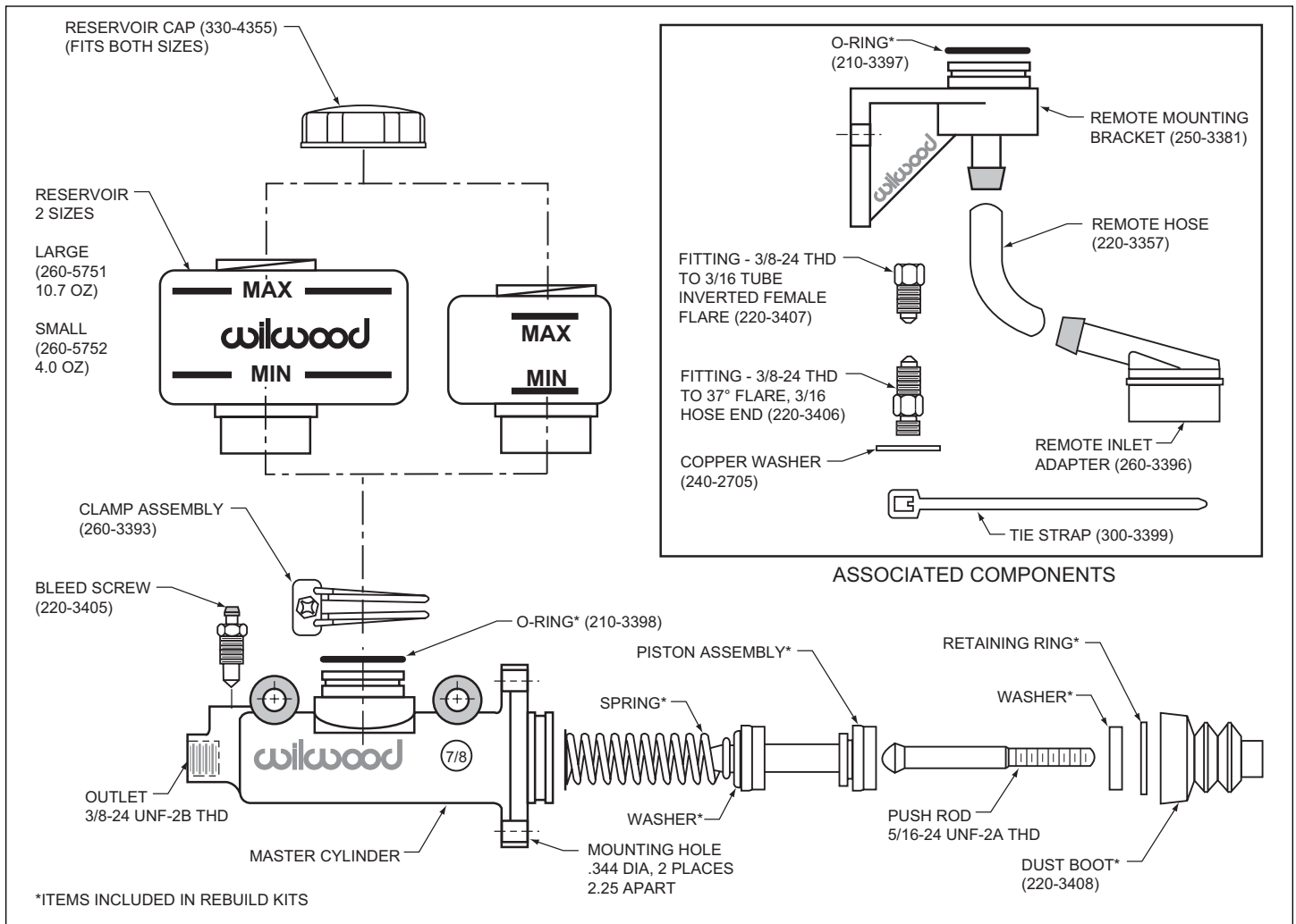
Figure 4. Master Cylinder and Associated Components
